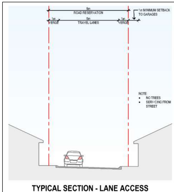
Figure 8 – Typical Section – Lane Access
