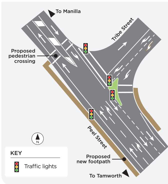
Design of new intersection at Peel Street (Manilla Road) and Tribe Street intersection
